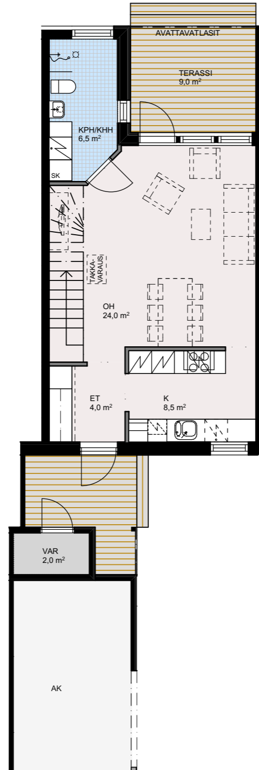
1.krs
