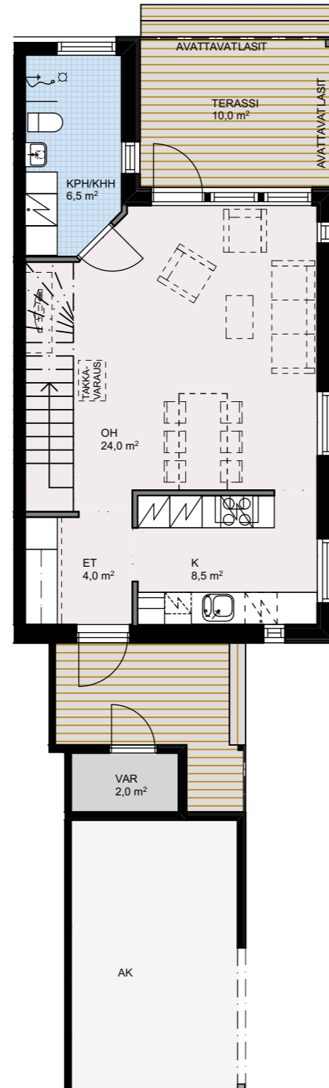
1.krs
