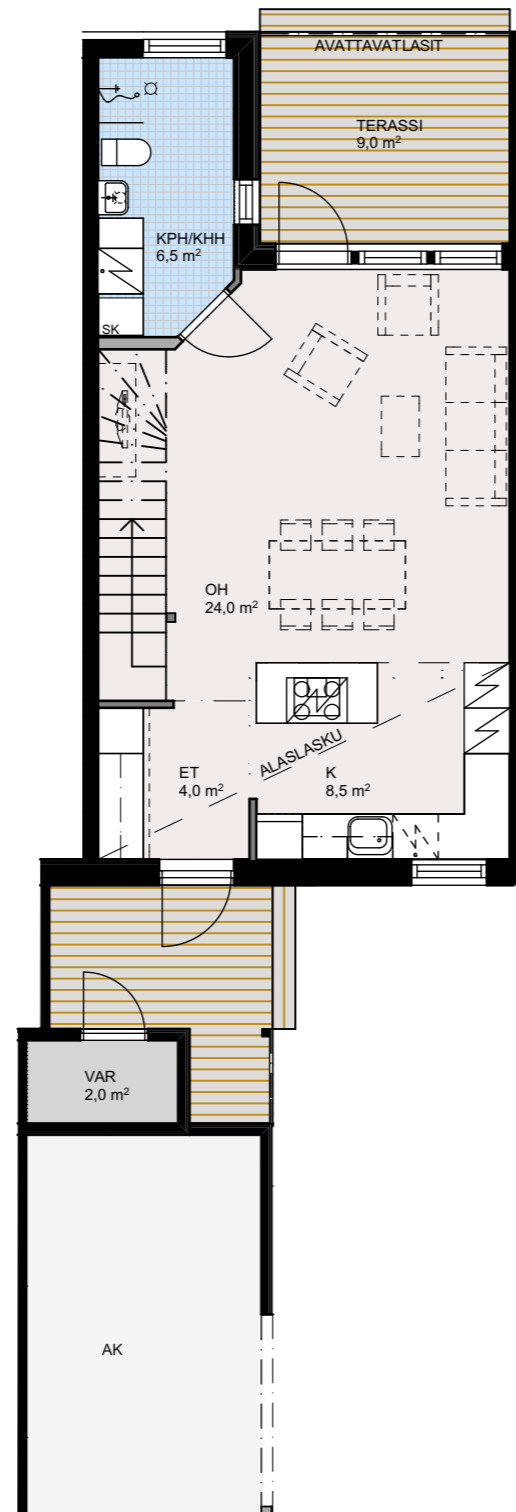
1.krs
