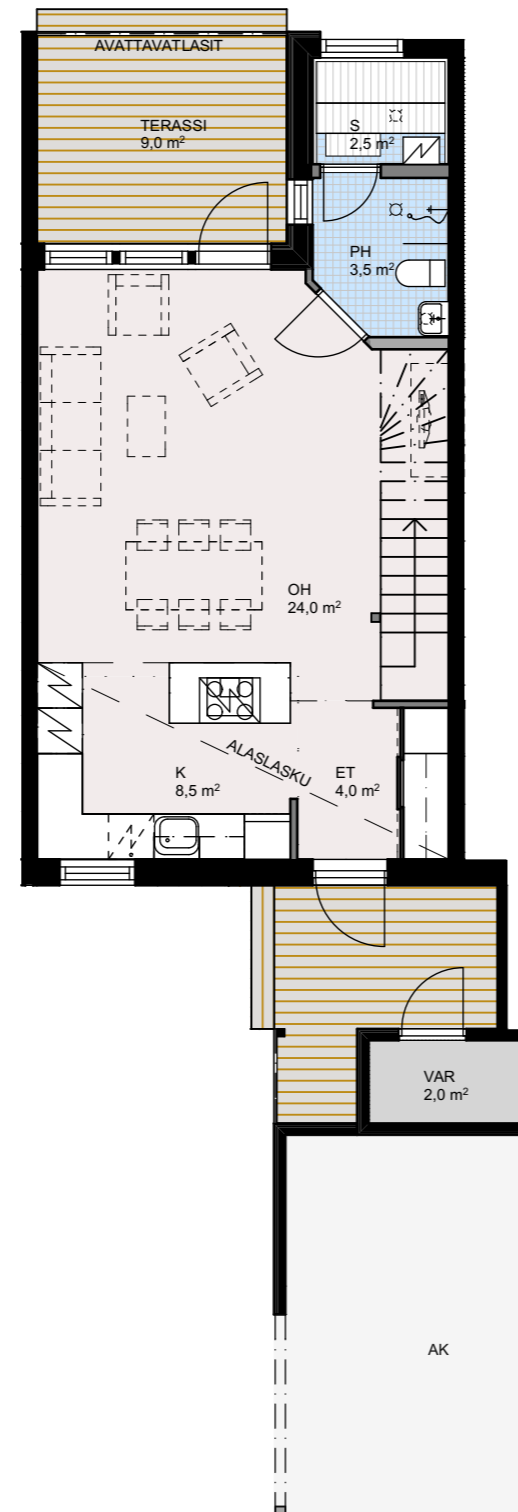
1.krs
